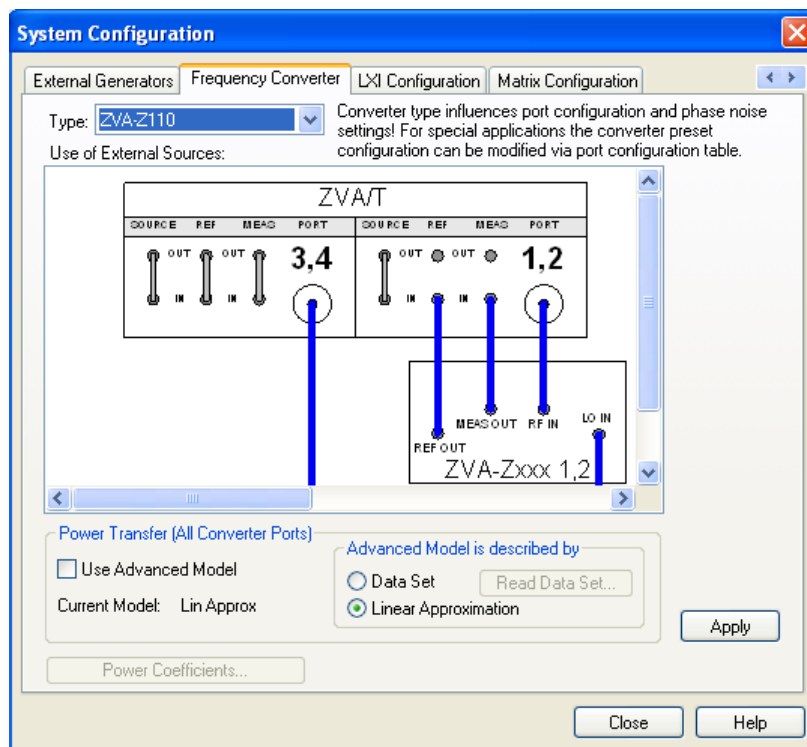
Fig. 3-1: Frequency Converter dialog (example: R&S ZVA-Z110)
