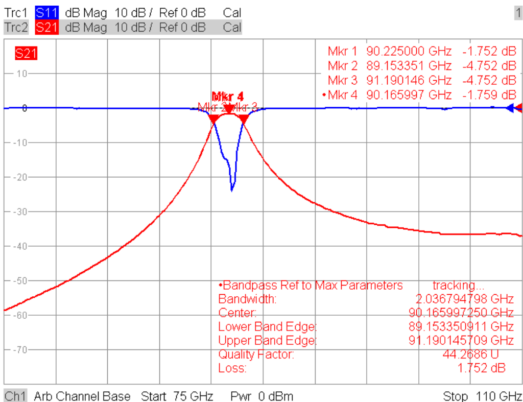
Fig. 3-2: Transmission and reflection of a bandpass filter measured with an R&S ZVA-Z110
