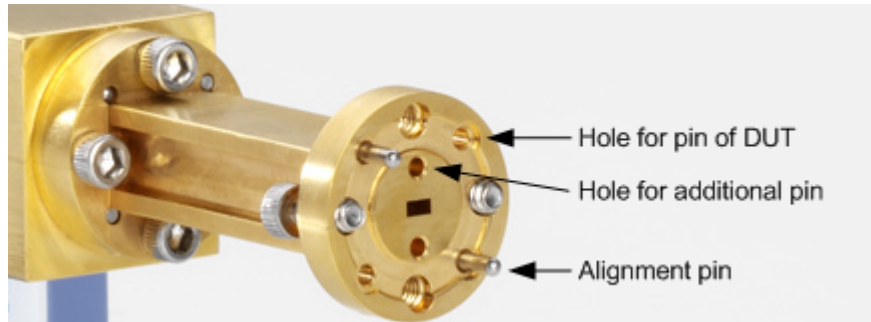
Fig. 2-2: Test port adapter of R&S ZVA-Z110
